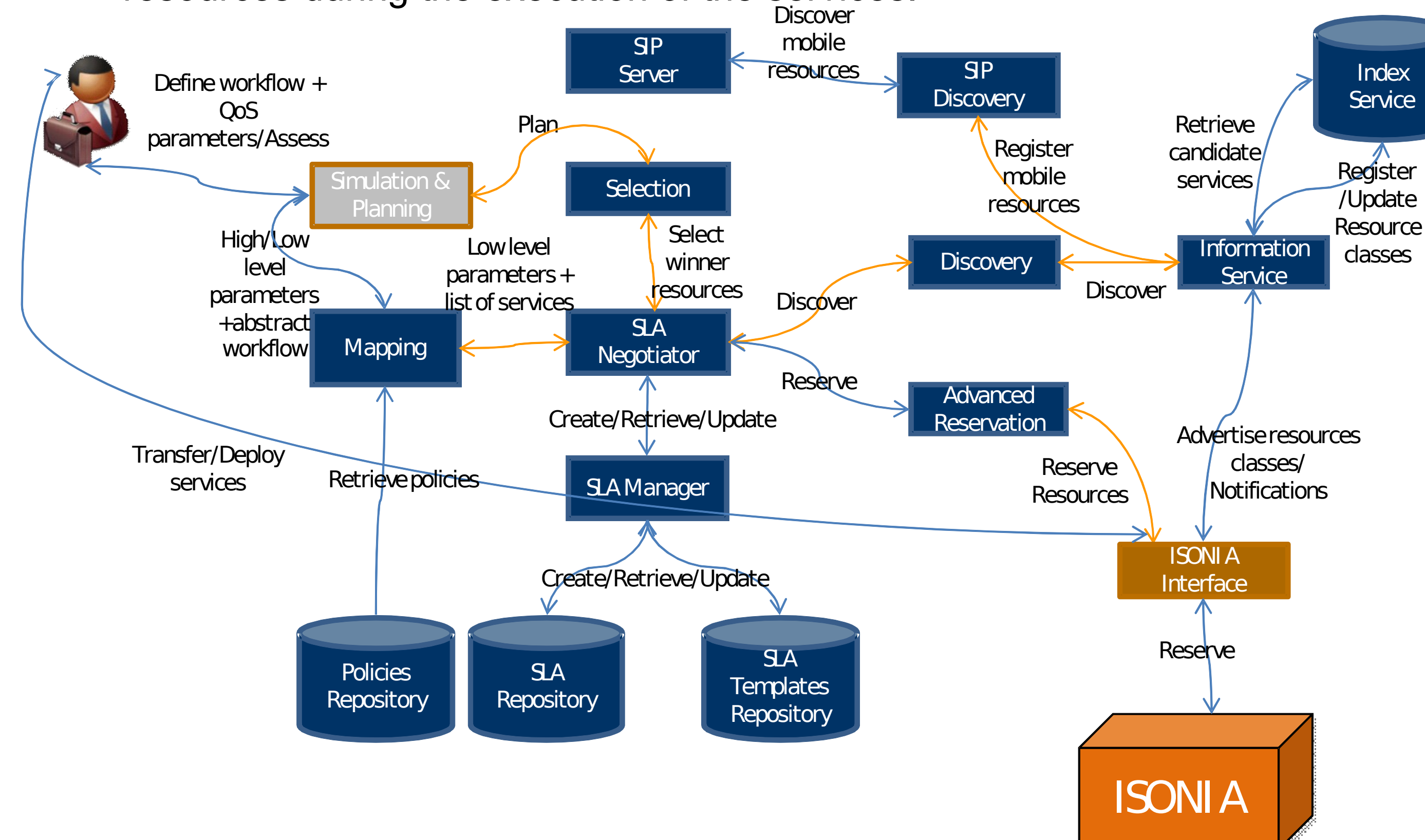
fig. 1: Component Model of Negotiation and Reservation Phase
