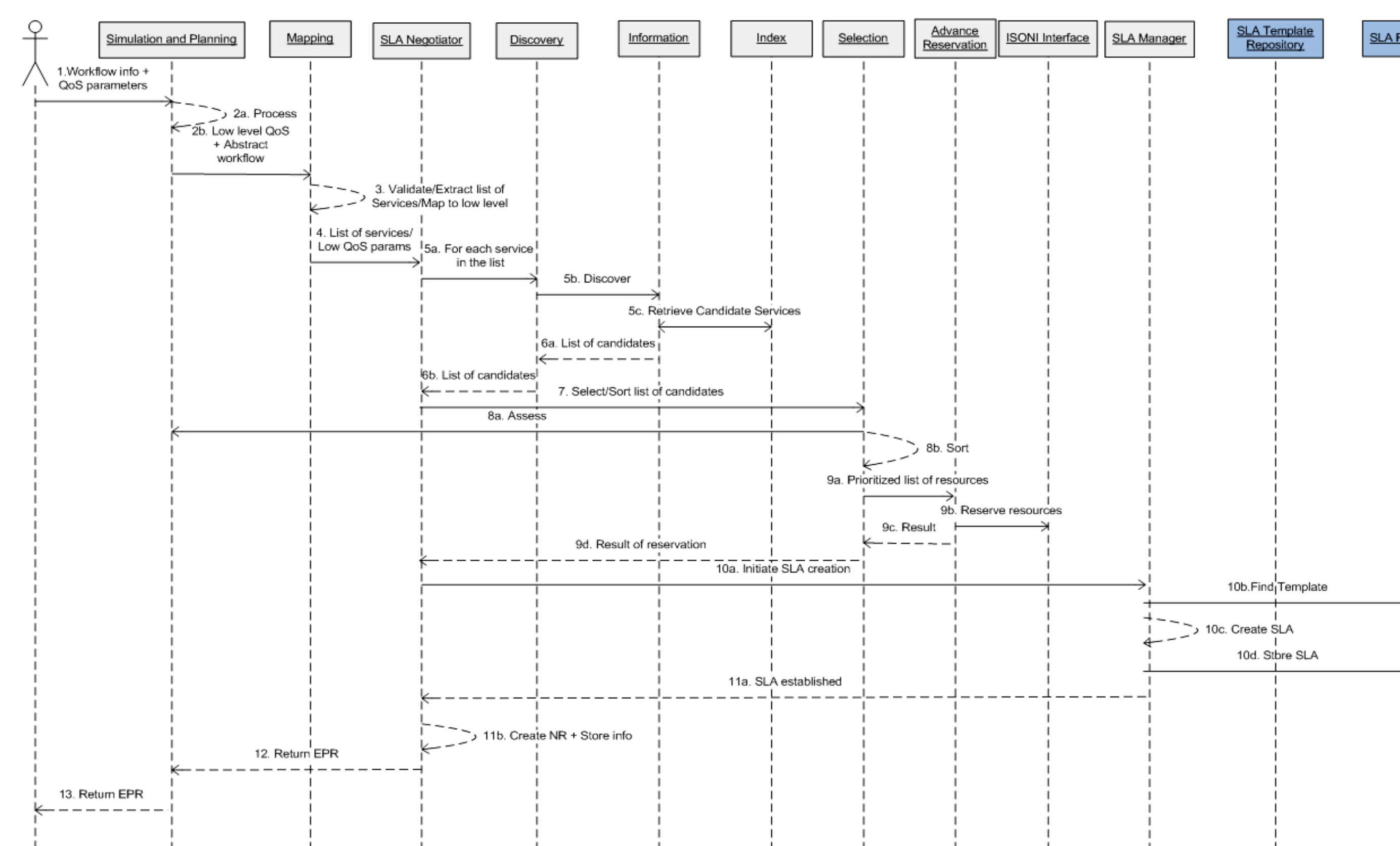
fig. 2: Sequence diagram for the Negotiation and Discovery phase
